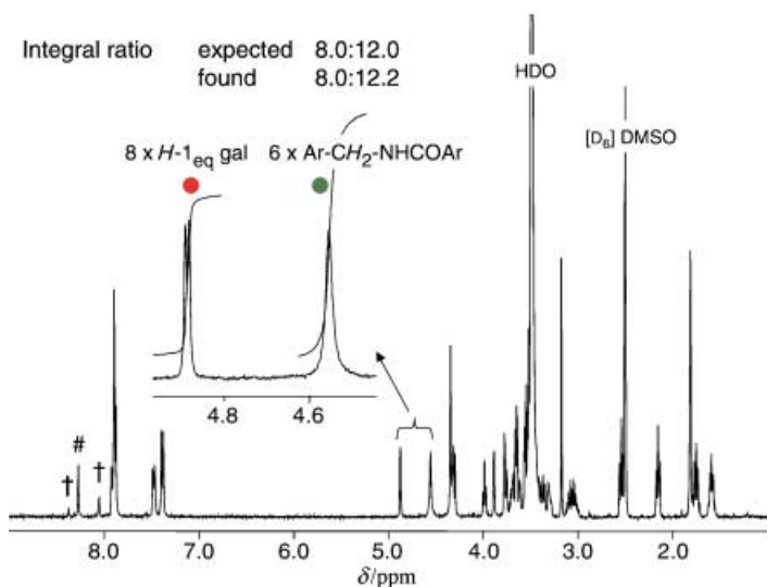
Figure 2. 500 MHz ^1\text{H} NMR spectrum of 3f (third generation, eight end groups) recorded in [\text{D}_6]\text{DMSO}/\text{D}_2\text{O} (5:1) at 75 °C. The spectrum demonstrates the remarkable purity (> 95 %) of this compound. The indicated signals represent 8 \times \text{H-1} of the terminal \alpha -linked galactose residue (see Scheme 1b, red) and 6 \times \text{Ar-CH}_2\text{-NHCO-Ar} of the dendrimer core (see Scheme 1a, green). Their relative intensities (8.0:12.2; expected 8.0:12.0) proves the quantitative functionalization with \alpha Gal. The small signals (indicated by †) at \delta = 8.05 ppm (intensity 1H) and \delta = 8.38 ppm (intensity 2H) can be assigned to the protons of the terminal trisubstituted ring of the dendrimer core structure, bearing the carboxylic acid functionality. The signal at \delta = 8.26 ppm (intensity 6H, indicated by #) reflects the protons between the N substituents of the six internal trisubstituted rings.
