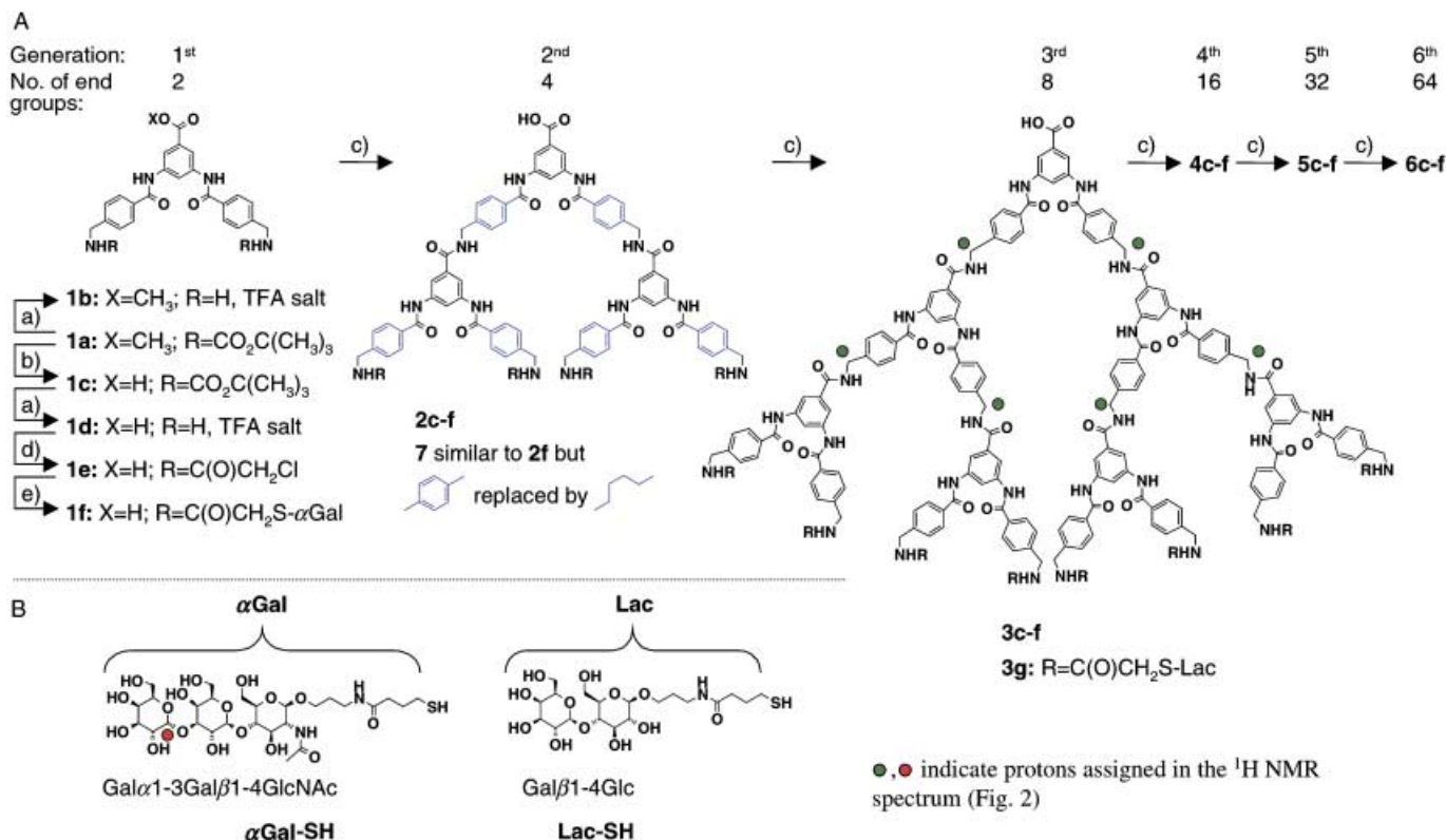
Scheme 1. A) Reaction conditions: a) TFA, \text{Et}_3\text{SiH} , \text{H}_2\text{O} (95:2.5:2.5), 3 h, RT (> 80 %); b) 1N NaOH/dioxane (1:1), 16 h, RT (82 %); c) 1) 1a (0.5 equiv), HBTU (1.0 equiv), DMF/ i\text{Pr}_2\text{NEt} (4:1), 6–16 h, RT; 2) LiOH, \text{H}_2\text{O} (> 75 %); d) chloroacetic acid anhydride (3.0 equiv), DMF/2,6-lutidine (3:1), 3 h, RT (50–95 %); e) \alpha Gal-SH or Lac-SH (1.5 equiv per end group), DMF, DBU, 1 h, RT; B) structures of \alpha Gal-SH and Lac-SH. TFA = trifluoroacetic acid, HBTU = O -(benzotriazol-1-yl)- N,N,N',N' -tetramethyluronium hexafluorophosphate, DMF = N,N -dimethylformamide
